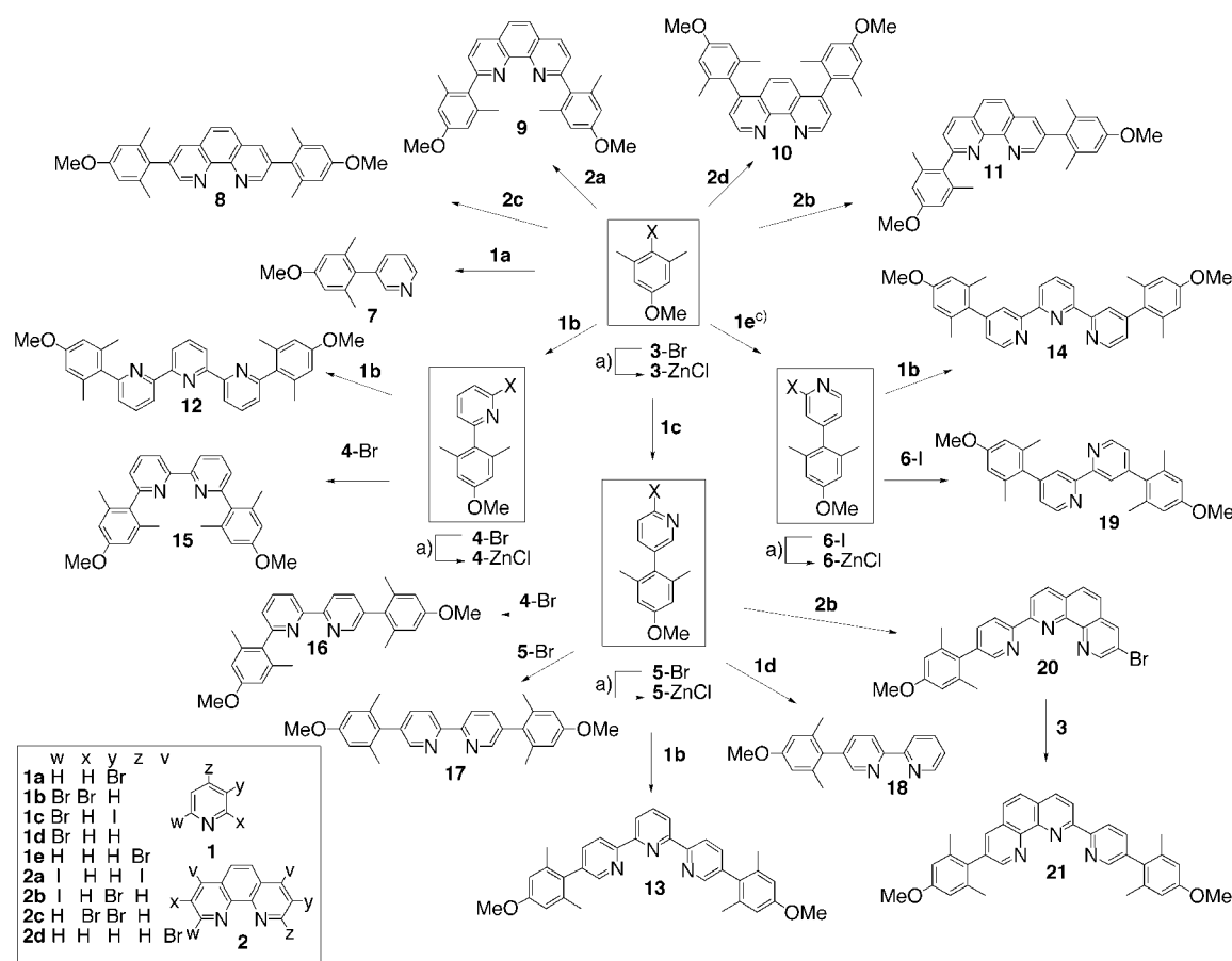
Scheme 1. a) n -Butyllithium, -78^{\circ}\text{C} , THF; \text{ZnCl}_2 , THF, -78^{\circ}\text{C} \rightarrow \text{RT} ; b) Aryl–X, 5% [\text{Pd}(\text{PPh}_3)_4] , reflux, 12 h, THF; c) see ref. [20].
